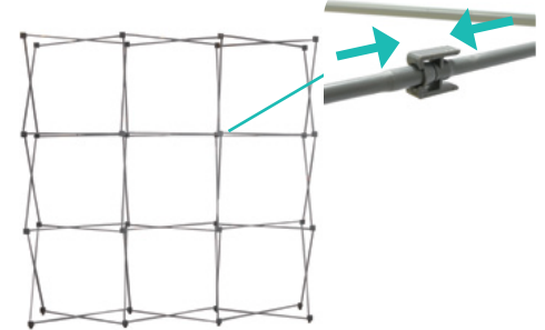
c. Close frame by pushing the outside of the frame until male and female ends connect.
