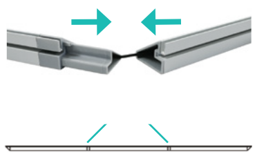
a. Expand each channel bar. Follow bungee to connect.
