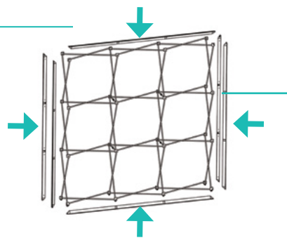
b. Attach channel bars to frame.
